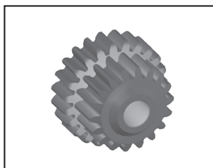
PD7222 2 SPEED PINION GEAR 齒輪18Tx23T
