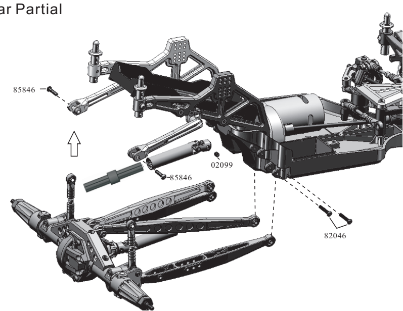
23. Rear Partial
