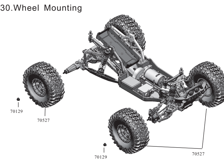
30. Wheel Mounting
