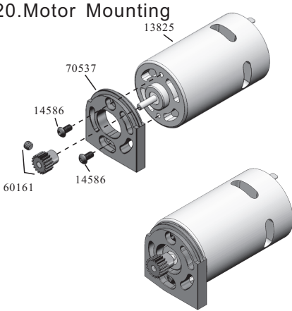
20. Motor Mounting
