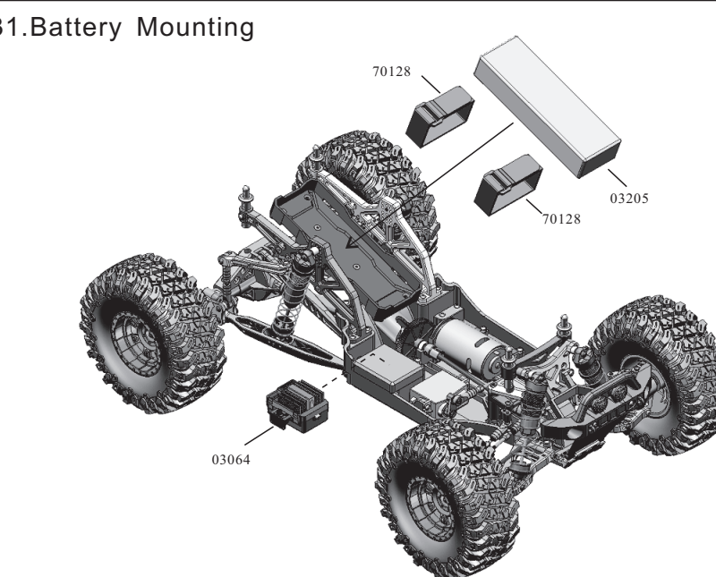
31. Battery Mounting
