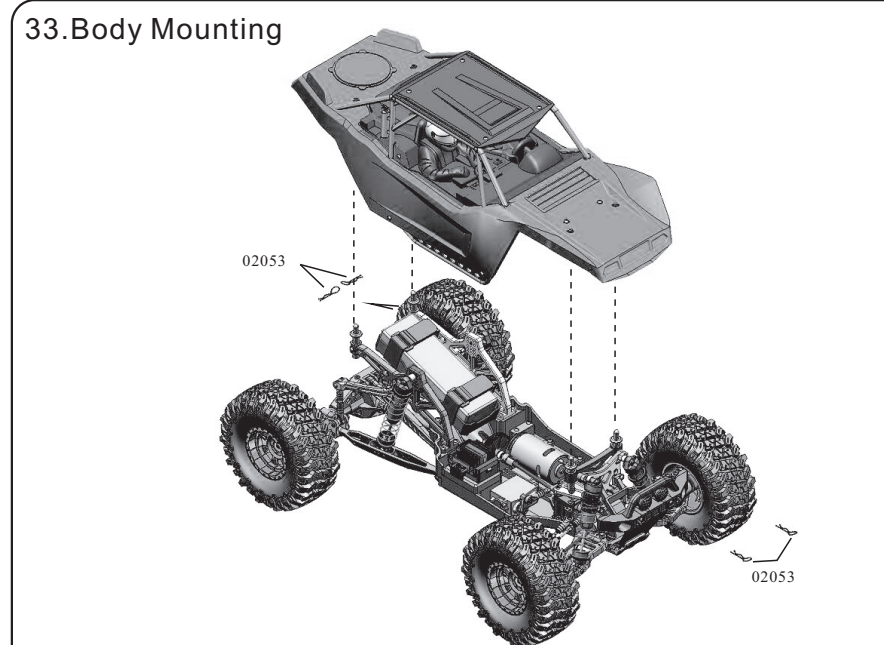
33. Body Mounting
