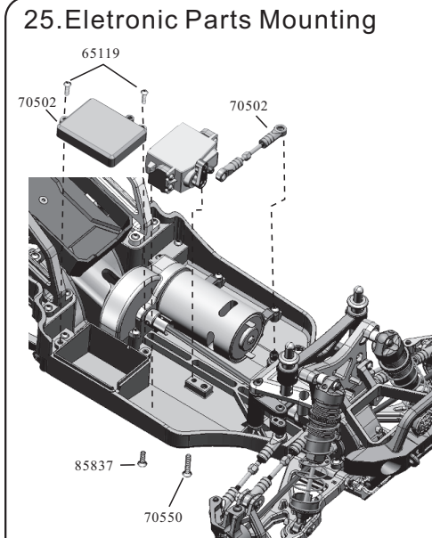
25. Electronic Parts Mounting
